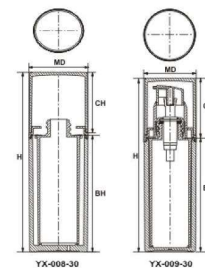
YX-008-30
