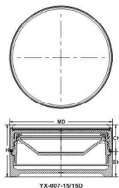
YX-007-15/15D
