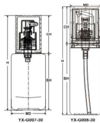
YX-G007-30
